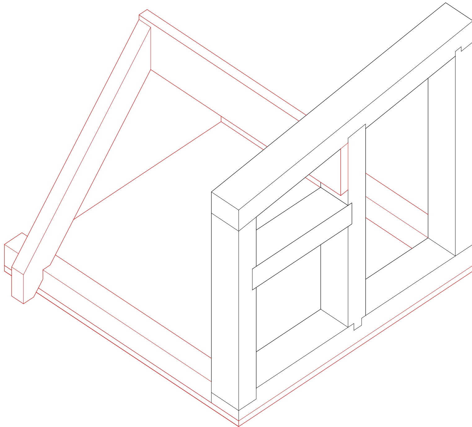
ISOMETRIC VIEW OF MODULE 1 & 2 MERGED
