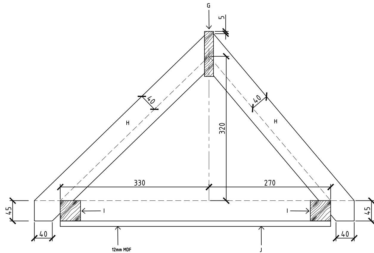
ROOF ELEVATION
